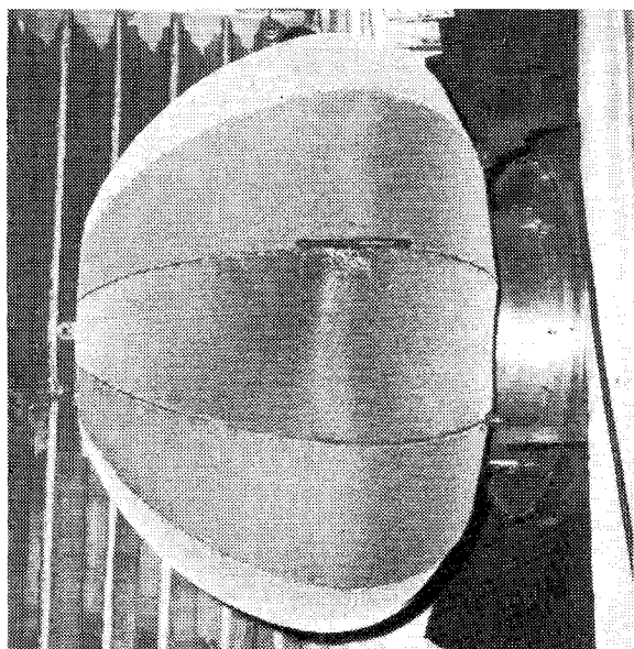
Fig. 6 View of the inflow control device installed in the LeRC anechoic chamber.
