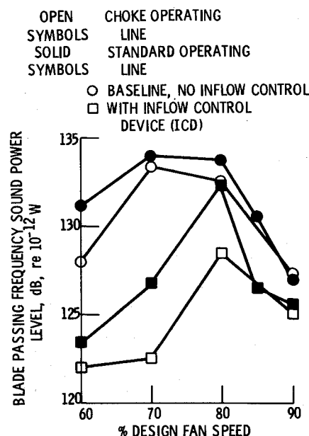
Fig. 14 Narrowband blade passing tone sound power level as a function of fan speed, 80 Hz bandwidth.
