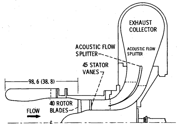
Fig. 3 Cross-sectional view of the research fan in the anechoic chamber and table of design parameters, cm (in.).
