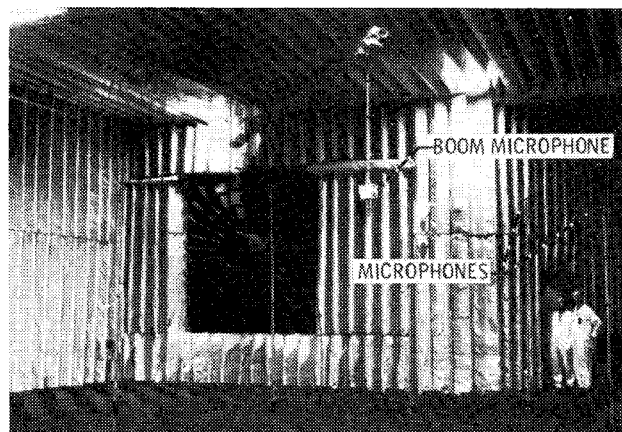
Fig. 1 Research fan installed in anechoic chamber.
