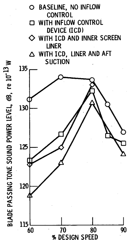
Fig. 12 Narrowband blade passing tone sound power level as a function of fan speed, standard operating line, 80 Hz bandwidth.
