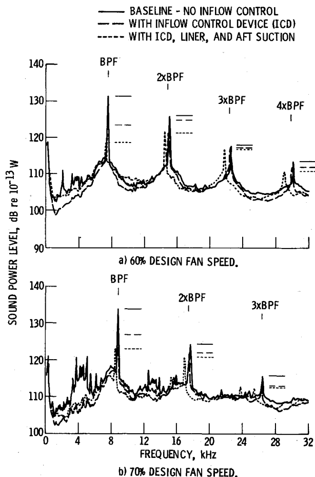
Fig. 8 Sound power level spectra, 80 Hz bandwidth, standard operating line.
