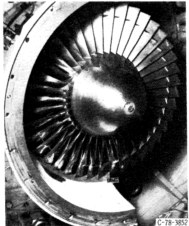
Fig. 4 View of partially assembled fan stage showing rotor blading.
