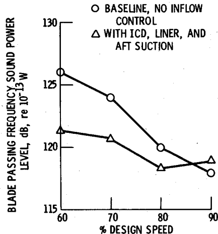
Fig. 15 Narrowband 1st overtone sound power level as a function of fan speed, standard operating line, 80 Hz bandwidth.
