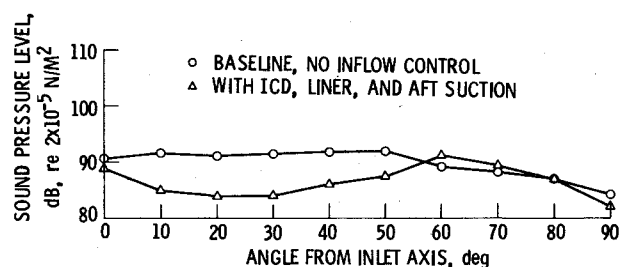
Fig. 13 Blade passing tone SPL directivity at 7.6 m (25 ft) radius, 90% design fan speed, standard operating line.
