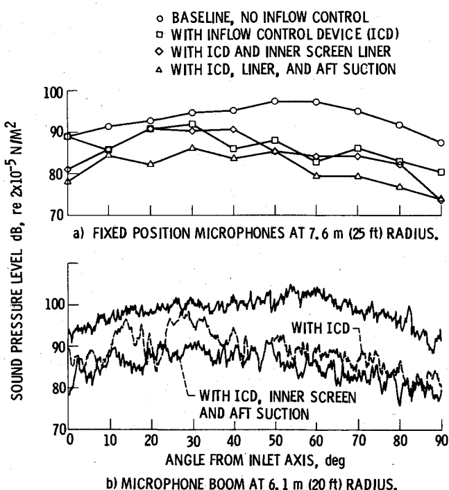
Fig. 9 Blade passing tone sound pressure level directivity, 60% design fan speed, standard operating line, 80 Hz bandwidth.
