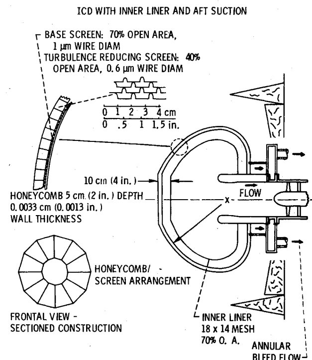
Fig. 5 Inflow control device showing inner screen liner and adaption of annular flow for aft suction.
