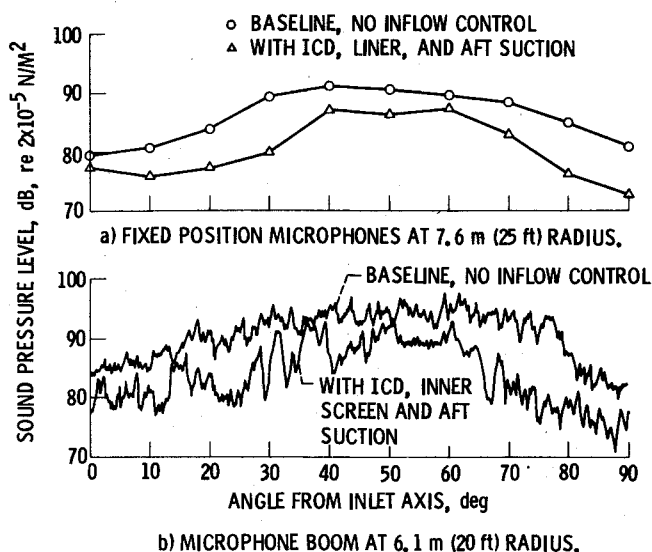
Fig. 11 First overtone ( 2 \times \text{BPF} ) sound pressure level directivity, 60% design fan speed, standard operating line, 80 Hz bandwidth.
