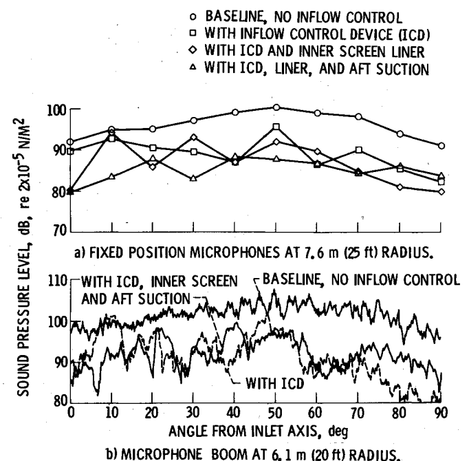
Fig. 10 Blade passing tone sound, pressure level directivity, 70% design fan speed, standard operating line, 80 Hz bandwidth.
